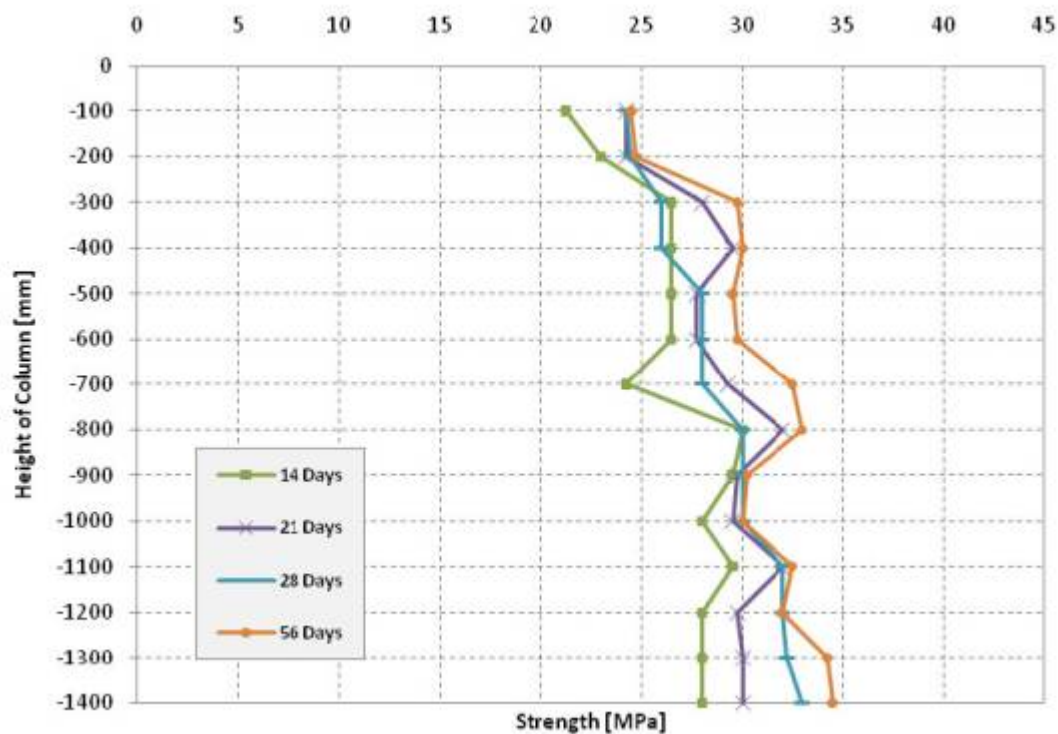
Figure C2: Column C2 - Cardboard Tube, Normal Concrete.
