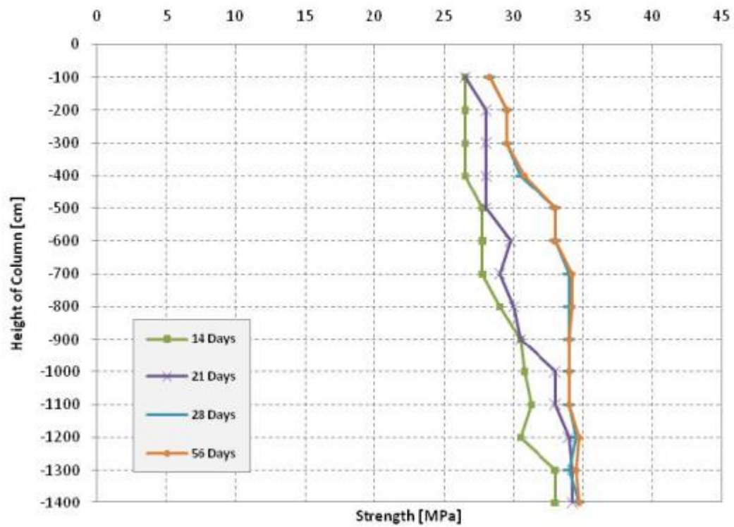
Figure C4: Column C4 - Cardboard Tube, Flyash Concrete.
