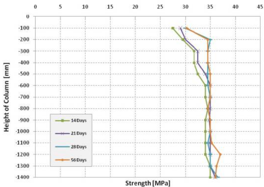
Figure C3: Column C3 - Fabric Formwork, Flyash Concrete.
