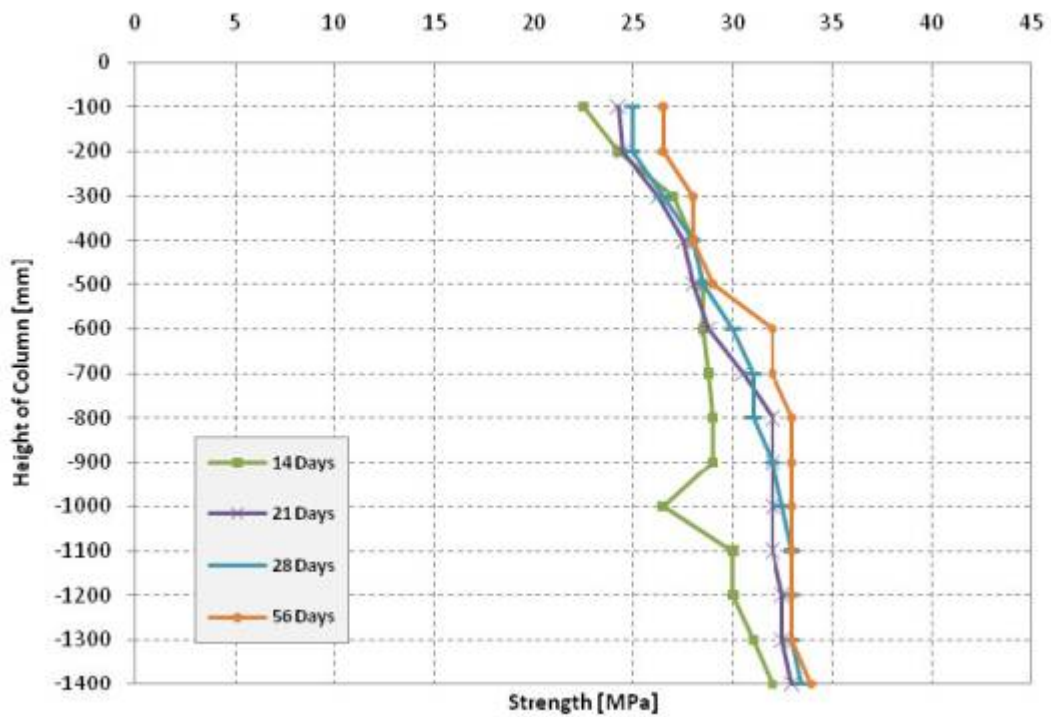
Figure C5: Column C5 - Fabric Formwork, Normal Concrete.
