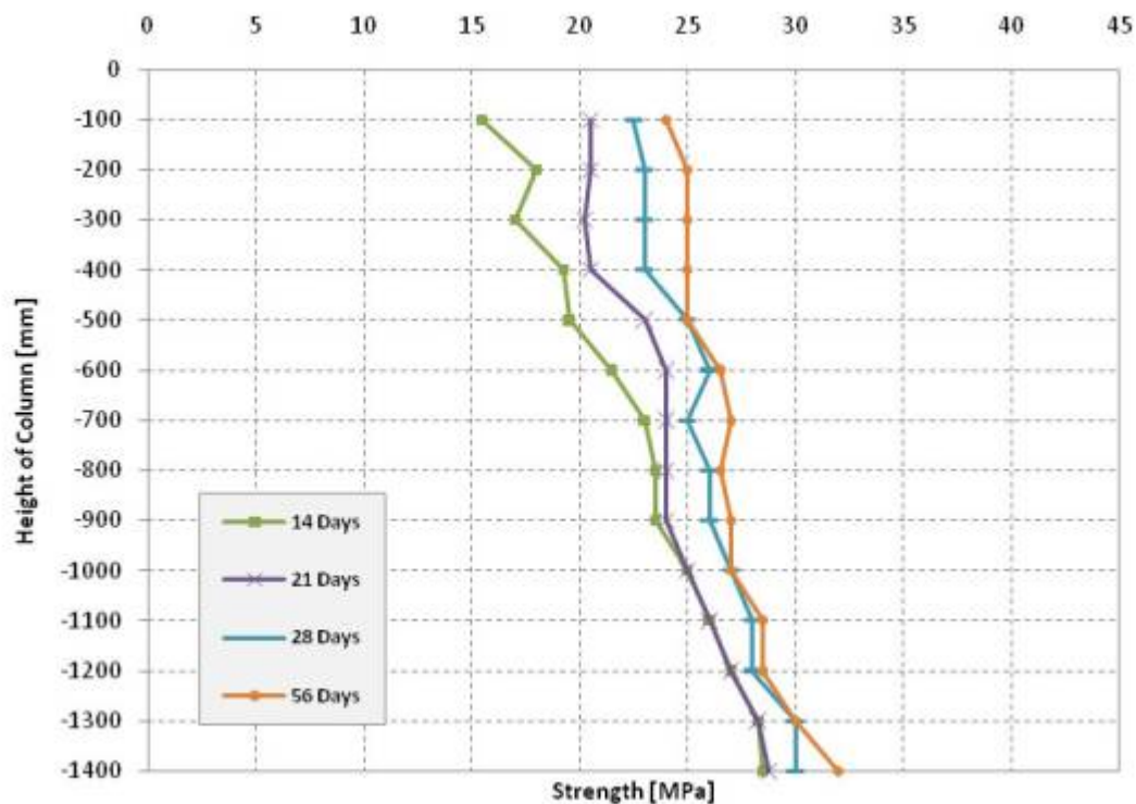
Figure C6: Column C6 – Cardboard Tube, Normal Concrete.
