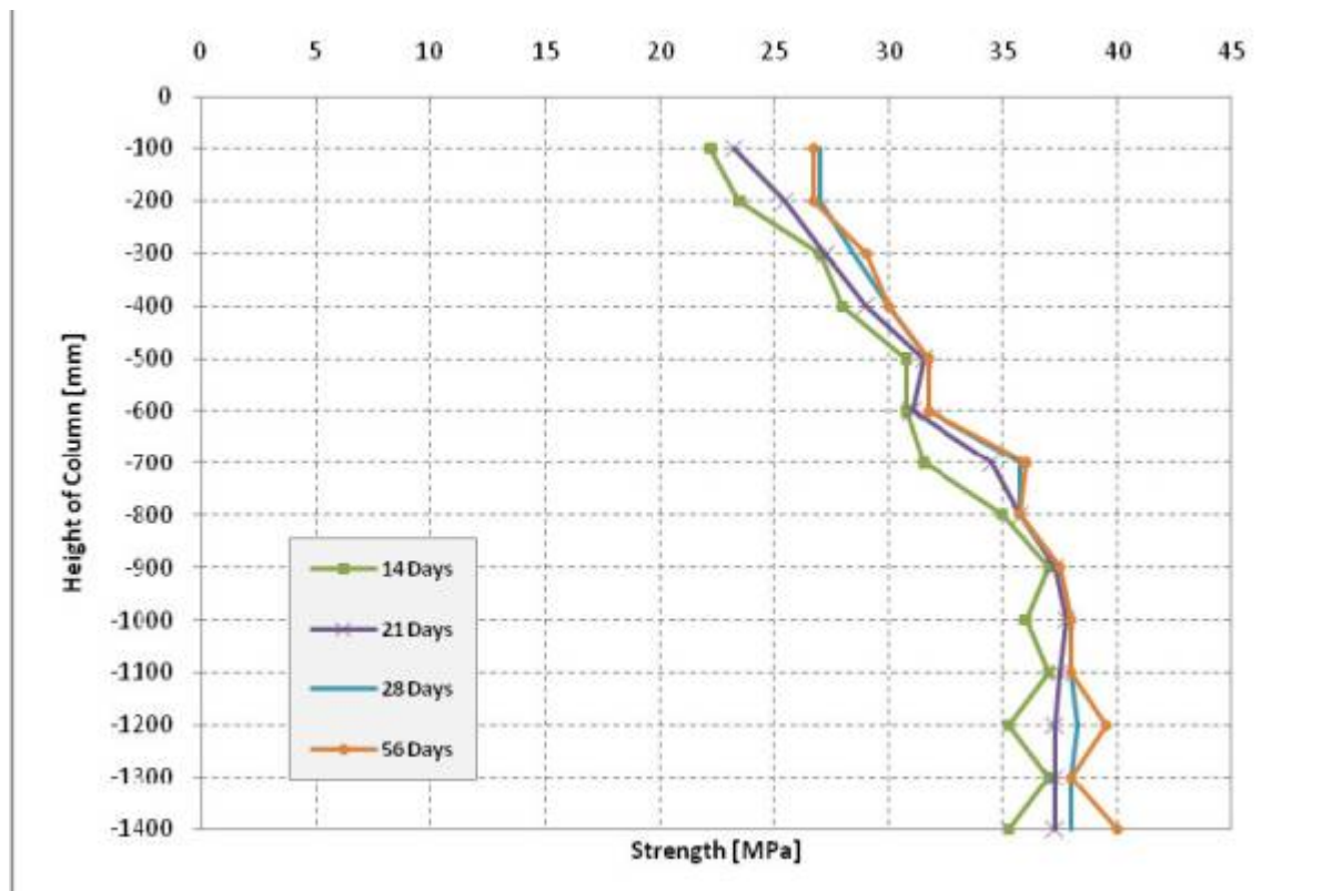
Figure C1: Column C1 – Fabric Formwork, Normal Concrete.
