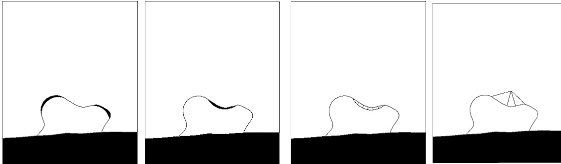
Fig 18: Wall locally strengthened around problem area.
