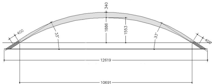
Figure 9: Pneumatic mould supported by the auxiliary structure (Tentech / Buitink Zeilmakerij).
