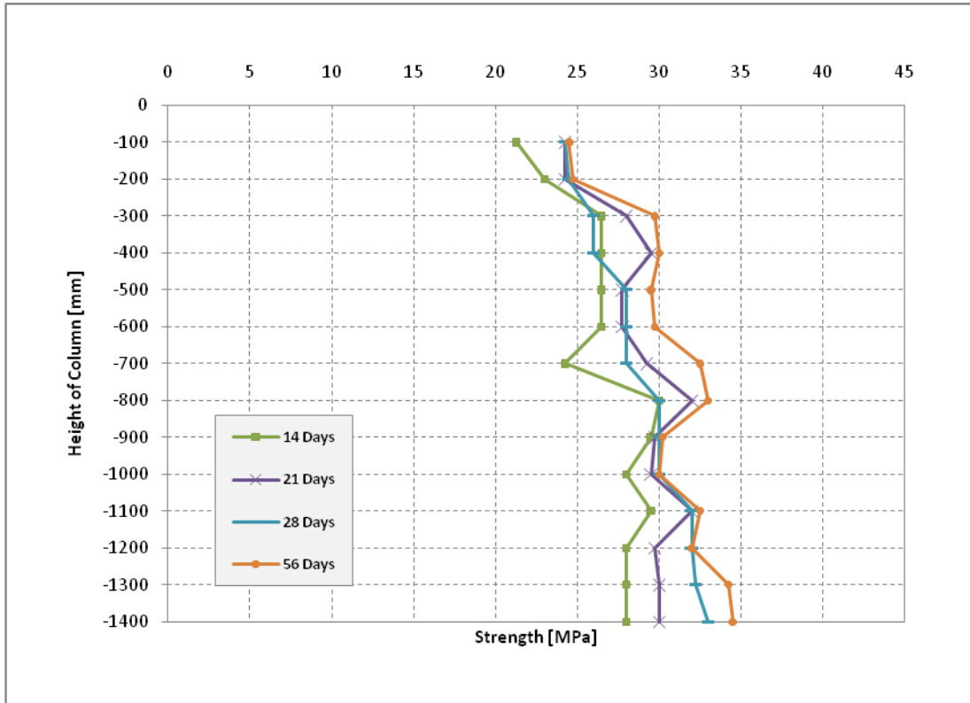
Figure C2: Column C2 – Cardboard Tube, Normal Concrete
