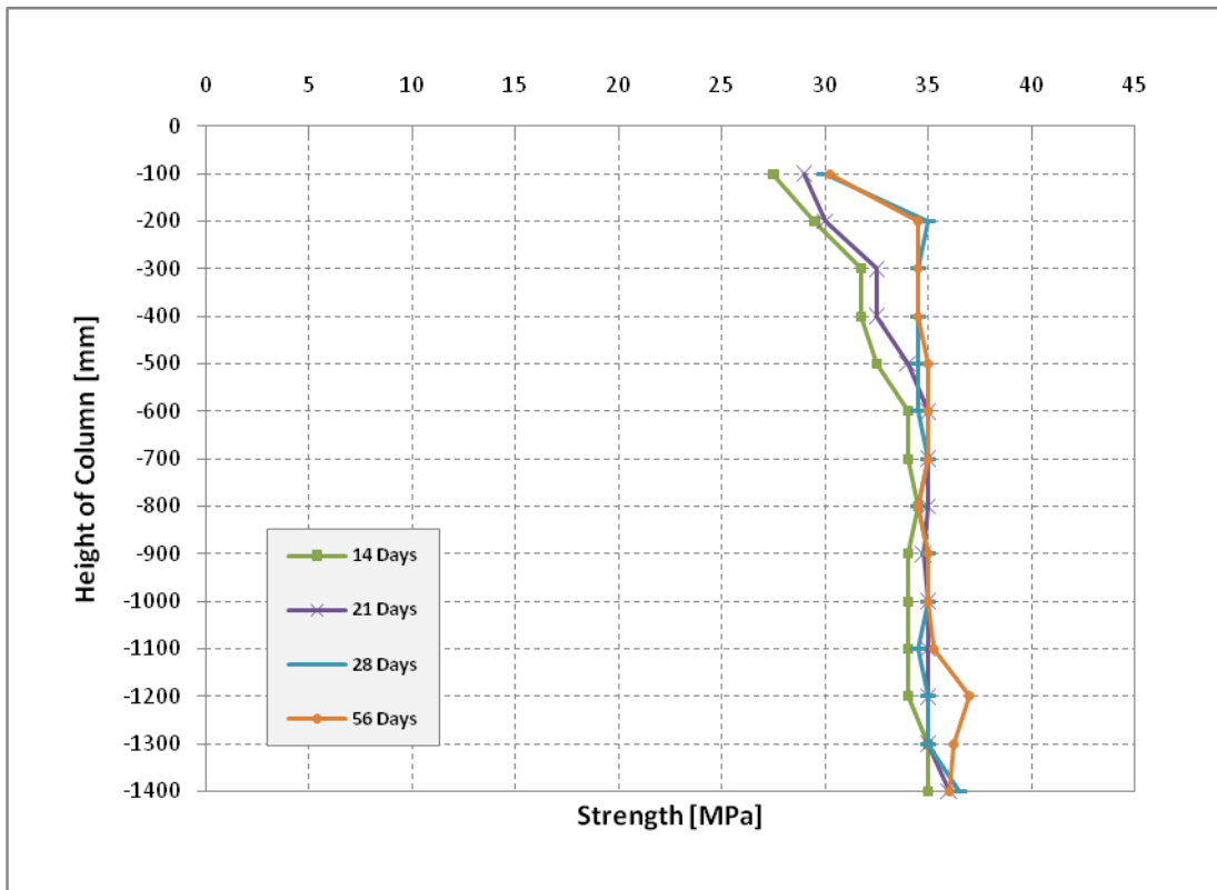
Figure C3: Column C3 – Fabric Formwork, Flyash Concrete
