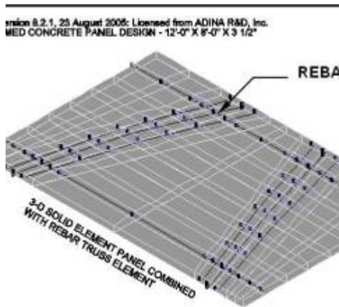
Fig. 21. Reinforced panel model.
