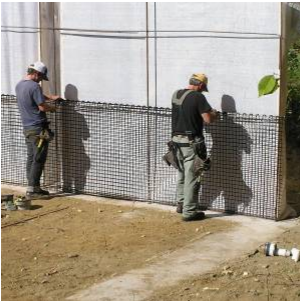
Adding Carbon Fiber Grid
