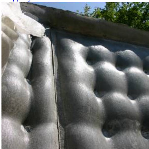
Stripping Formwork
