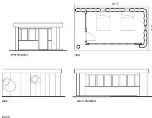
The "Pillow Cabin" Plans
