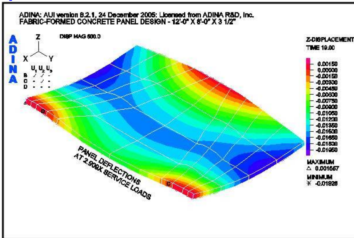
Fig. 12. Panel model.
