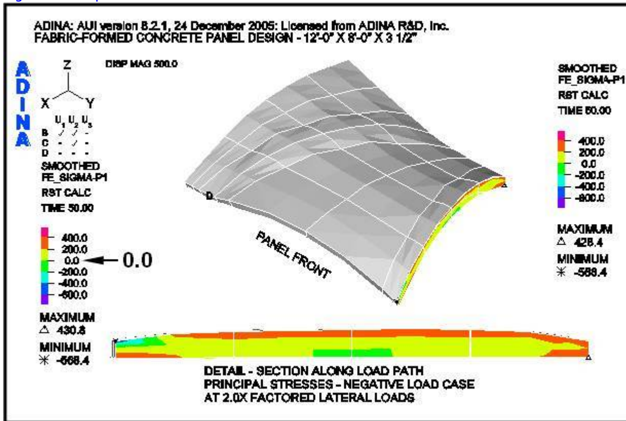
Fig. 20. Principal stresses at section cut.
