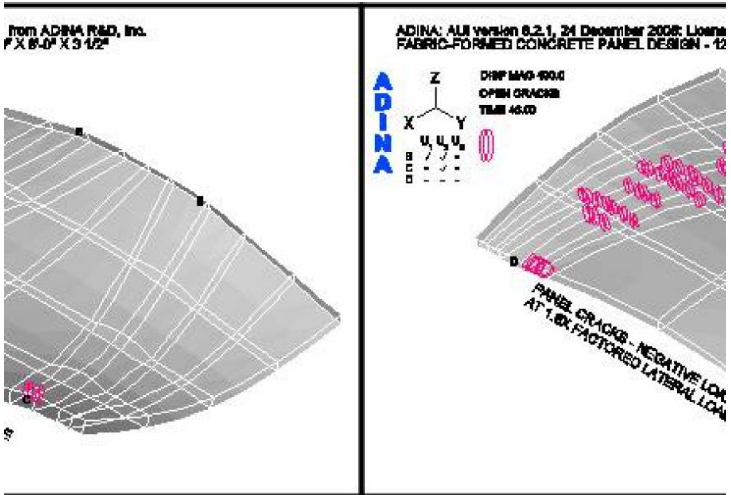
Fig. 18c. Progression of panel crack patterns, back (left) and front (right).
