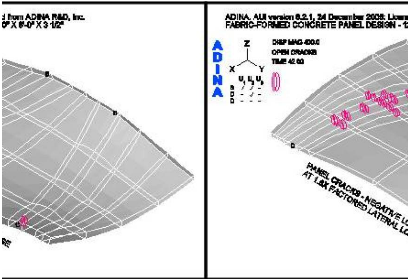
Fig. 18b. Progression of panel crack patterns, back (left) and front (right).
