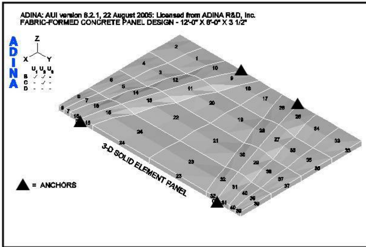
Fig. 12. Panel model.
