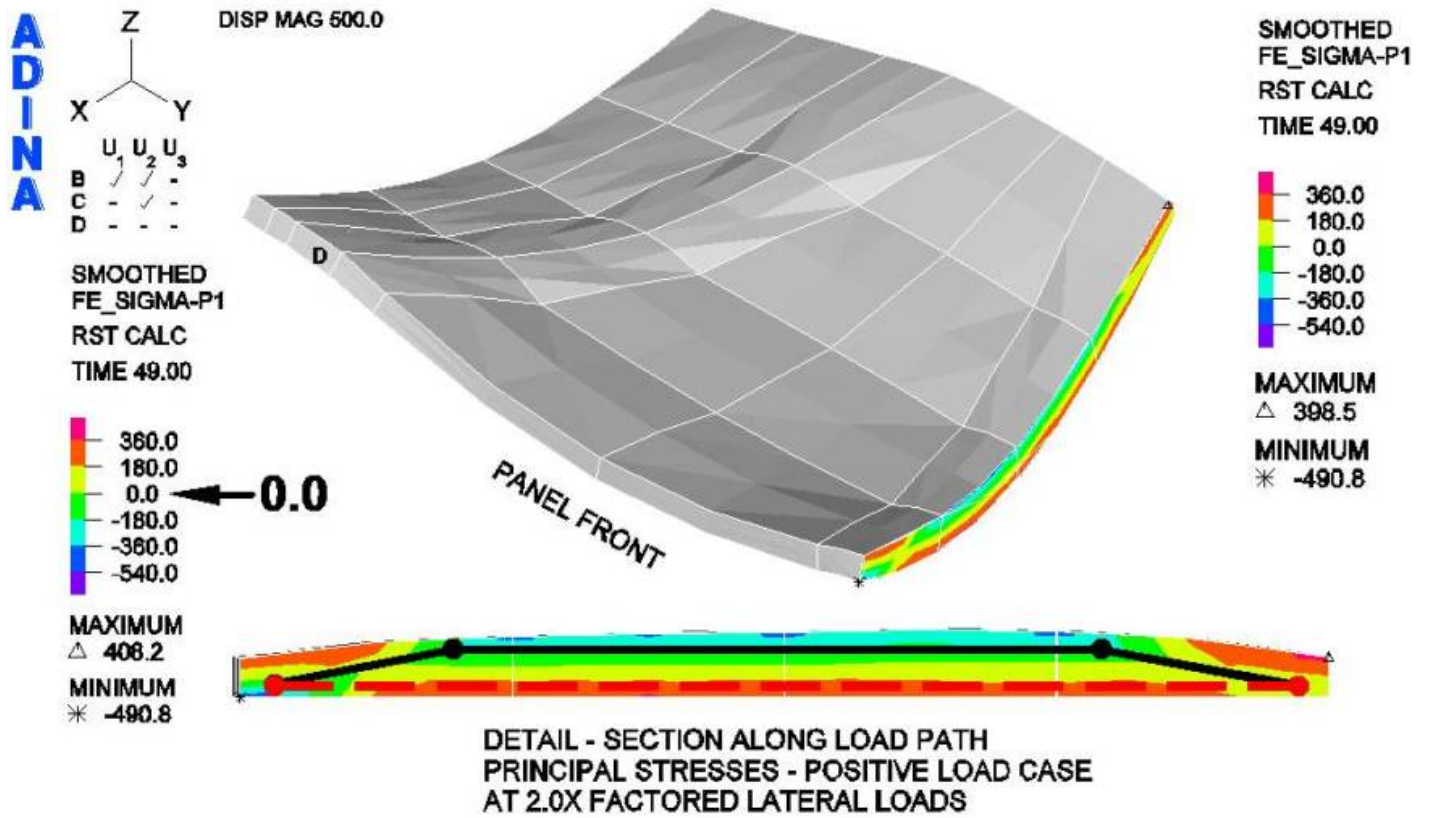
Fig. 19. Principal stresses at section cut.
