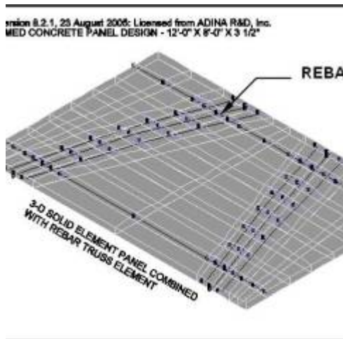
Fig. 21. Reinforced panel model.
