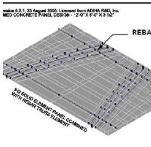
Fig. 21. Reinforced panel model.
