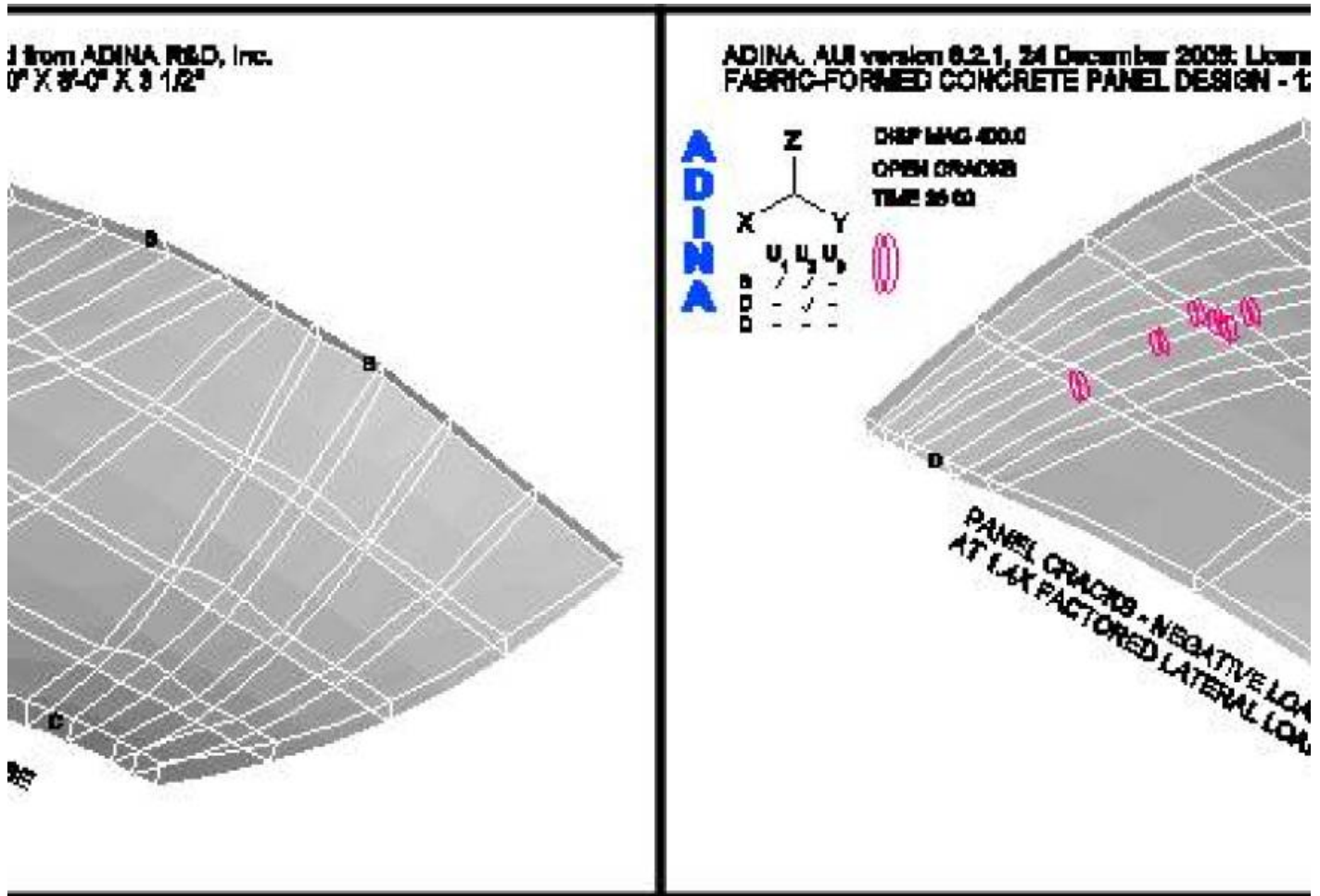
Fig. 18a. Progression of panel crack patterns, back (left) and front (right).
